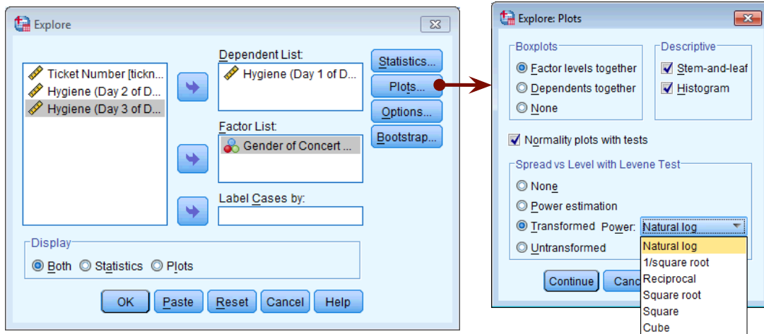
Figure 11: Exploring groups of data and obtaining Levene’s test
